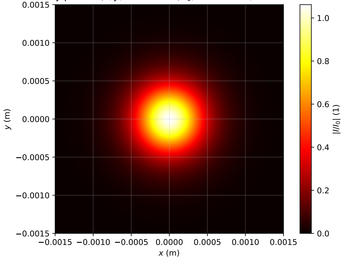
Intensity profile I(x, y, z = 1.513m)/I_0 , P_{in}=0.6P_{cr} , artificial time
